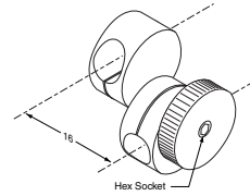
53-3869 Duel swivel clamp, dual 1/2 inch posts
